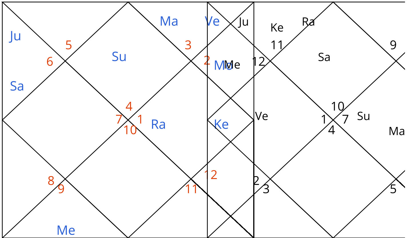
Vimsamsa (D-20)
