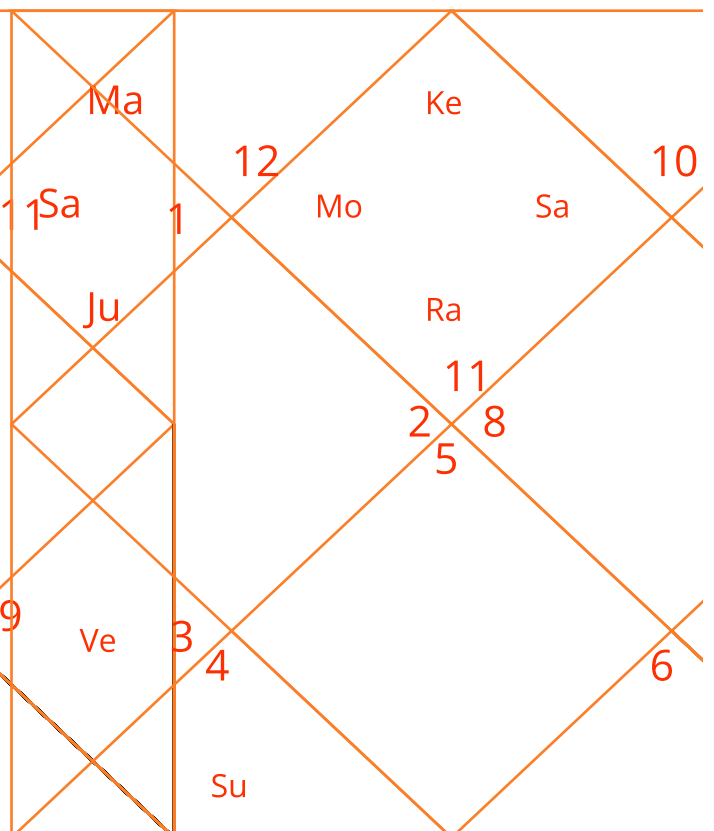
Akshavedamsa (D-45)
